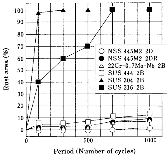
Fig. 3. Variation in Rust Area with Time After Weather Simulated Corrosion Test
