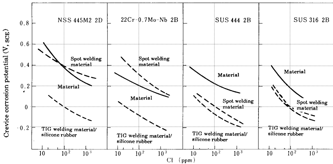
Fig. 2. Relationship between Crevice Corrosion Potential and Cl - Concentration in Diluted Salt Solution (at 80°C)
